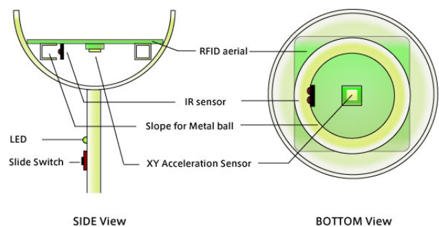
Figure 1. Maracas based device configuration diagram.
